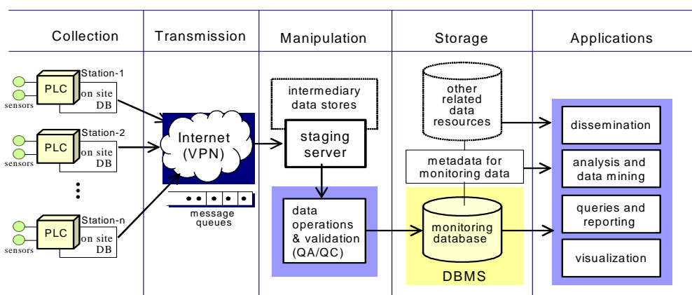
Figure 2.1: System architecture for environmental monitoring data management – ranging from data collection to data applications
