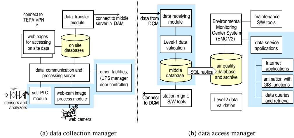
Figure 3.1: TAQMN-2 overall structures
